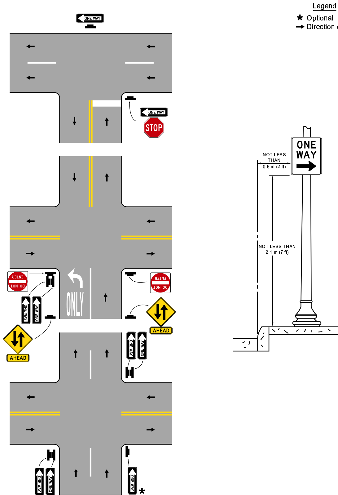
Figure 2B-12. Examples of Locations of ONE WAY Signs (Sheet 2 of 2)
