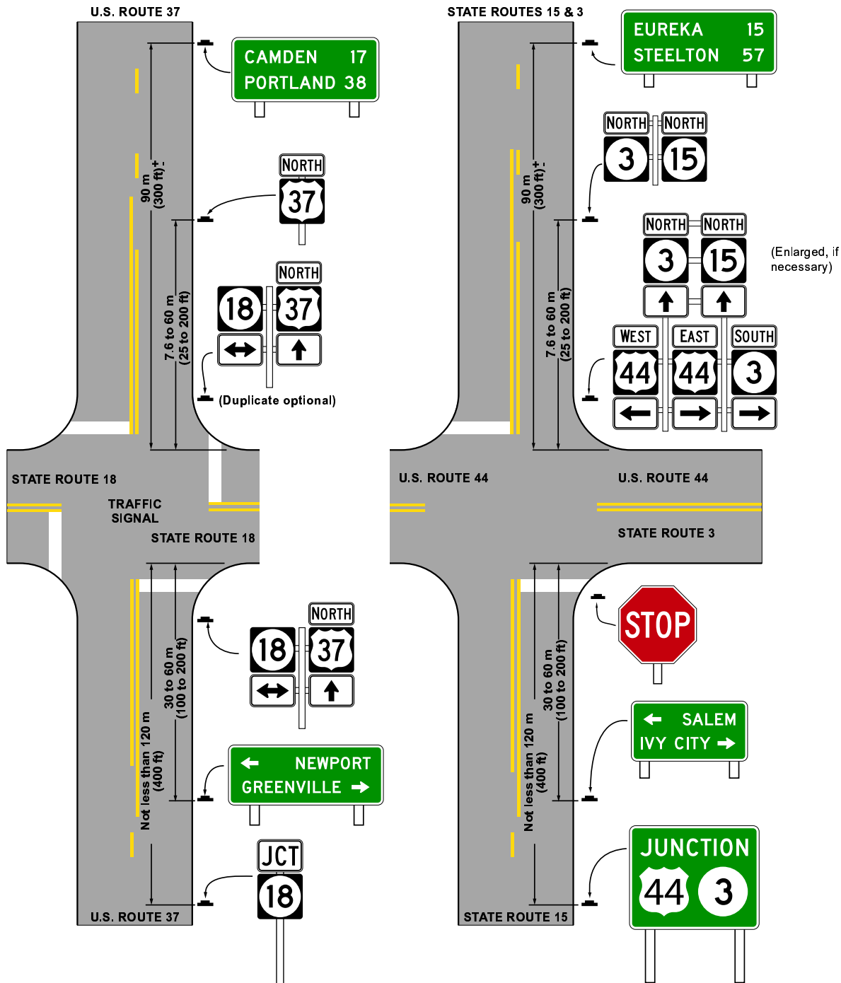
Figure 2D-6. Illustration of Directional Assemblies and Other Route Signs (For One Direction of Travel Only) (Sheet 1 of 3)
