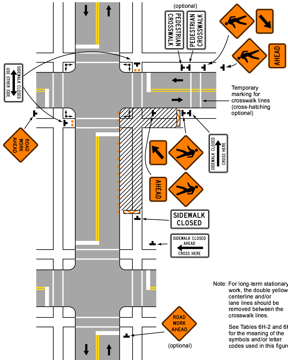
Typical Application 29
