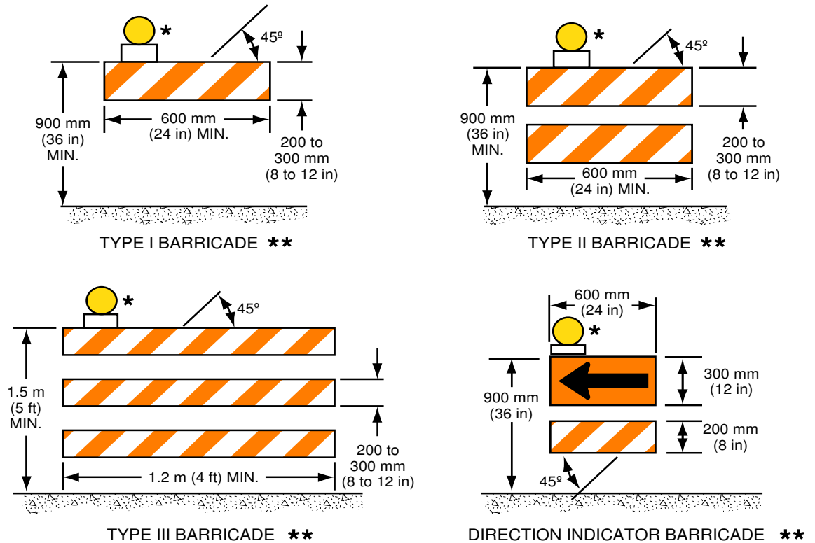
Figure 6F-7. Channelizing Devices (Sheet 2 of 2)
