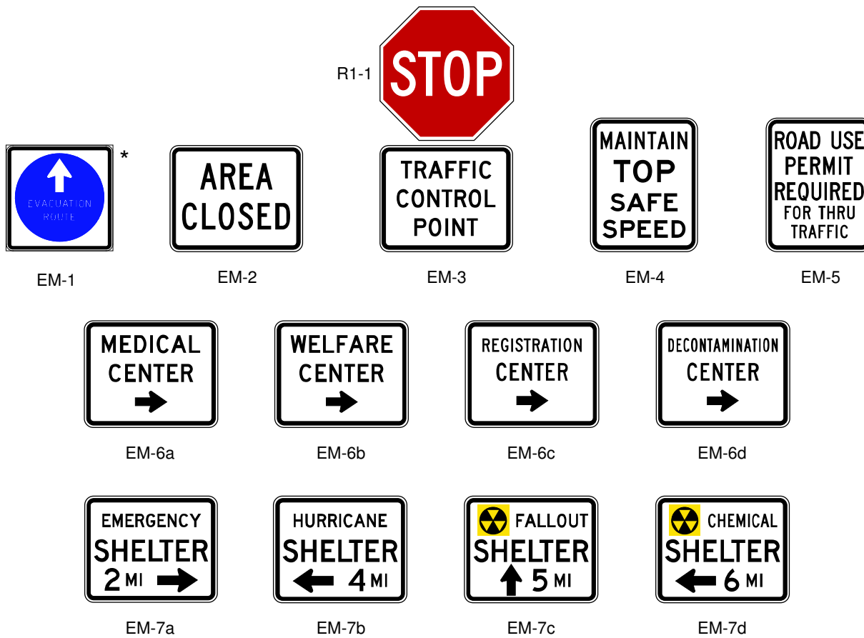
Figure 2I-1. Emergency Management Signs
