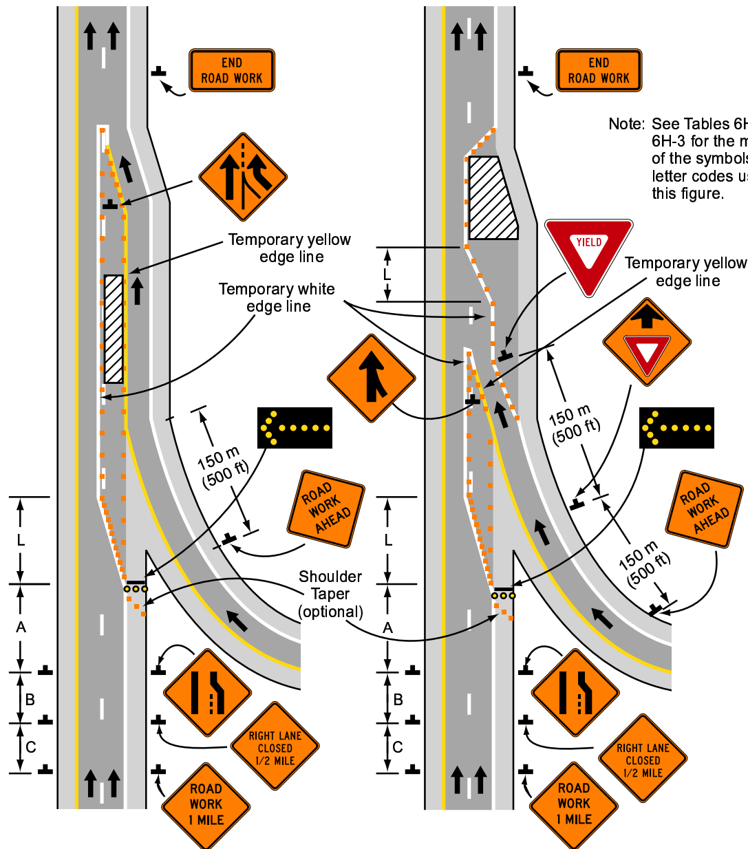
Typical Application 44
