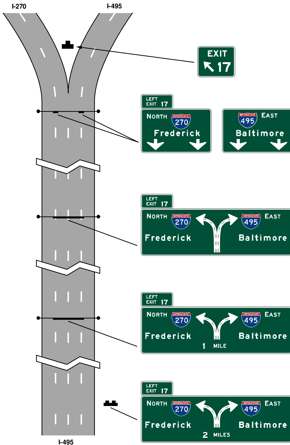
Figure 2E-4. Diagrammatic Signs for Split with Dedicated Lanes
