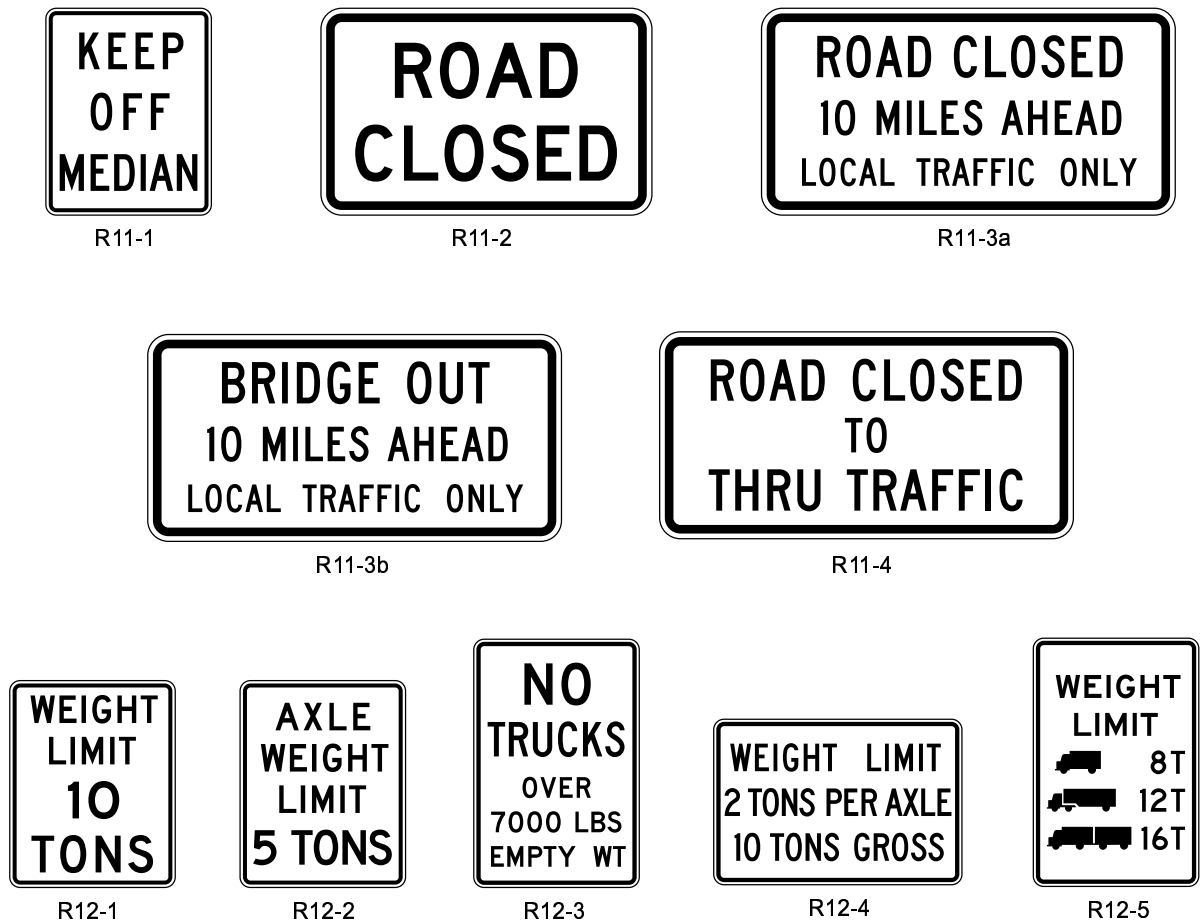
Figure 2B.20. Road Closed and Weight Limit Signs
