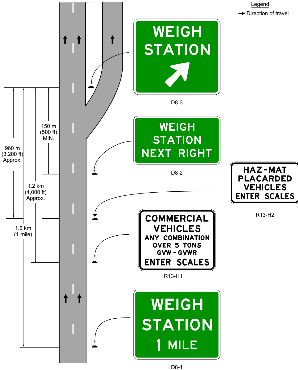
Figure 2D-10. Example of Weigh Station Signing
