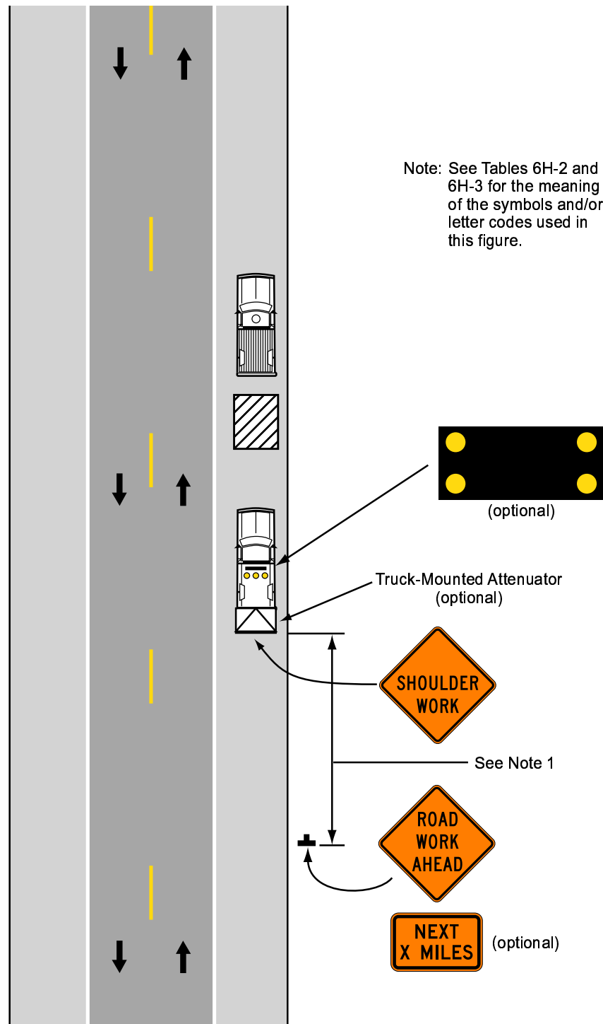
Typical Application 4
