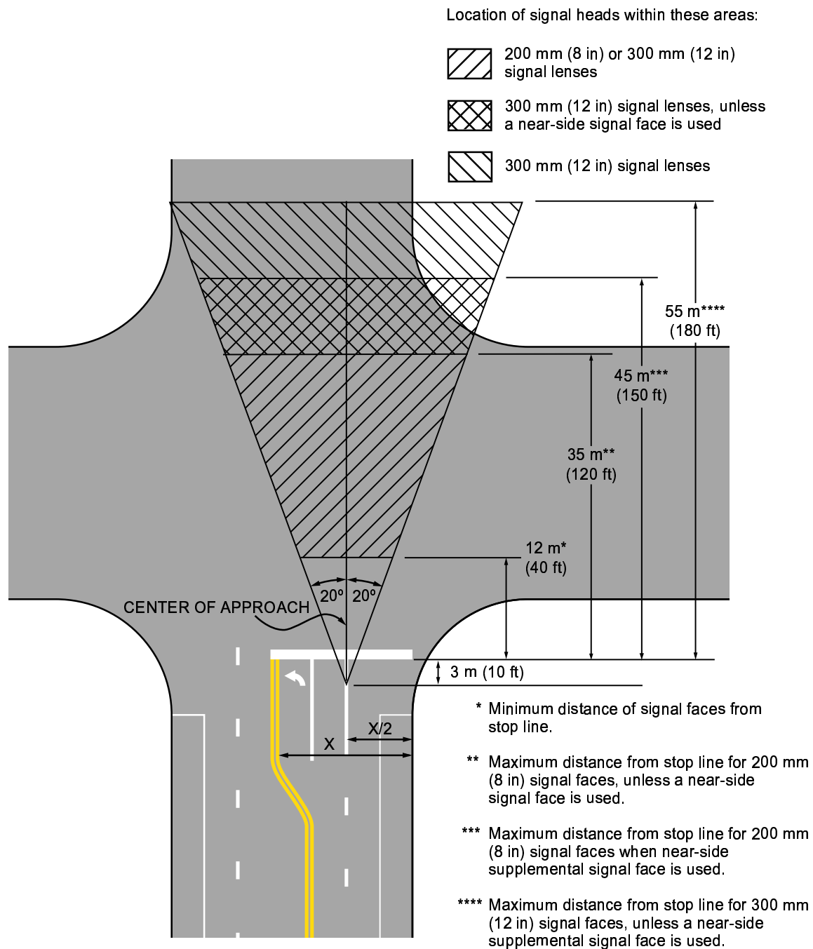
Figure 4D-2. Horizontal Location of Signal Faces
