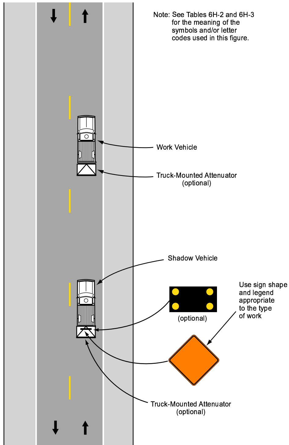
Typical Application 17
