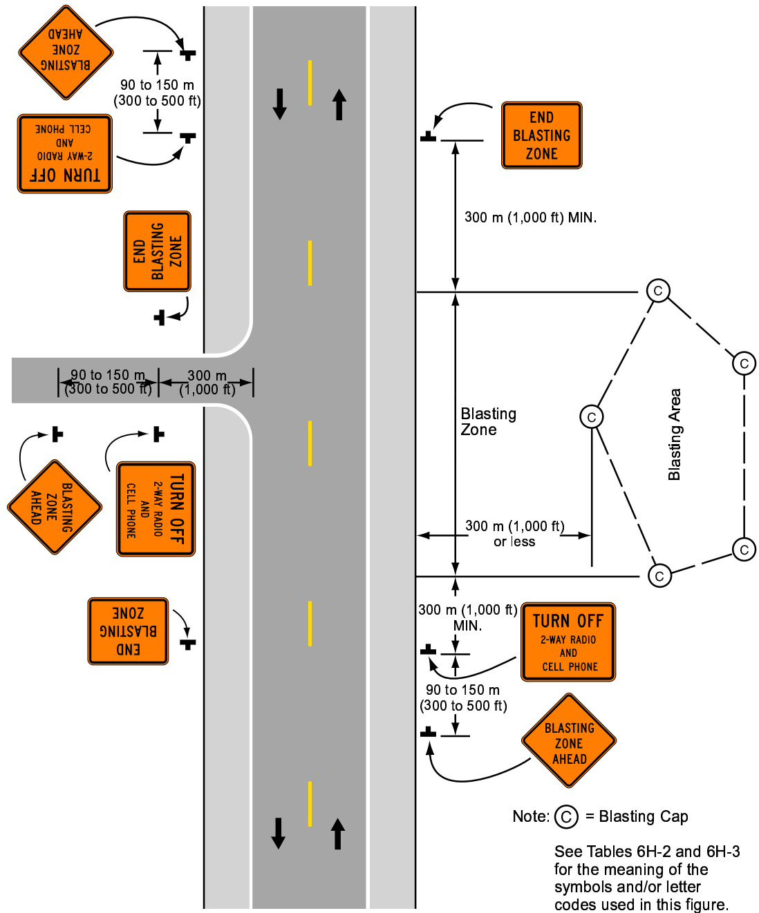
Typical Application 2
