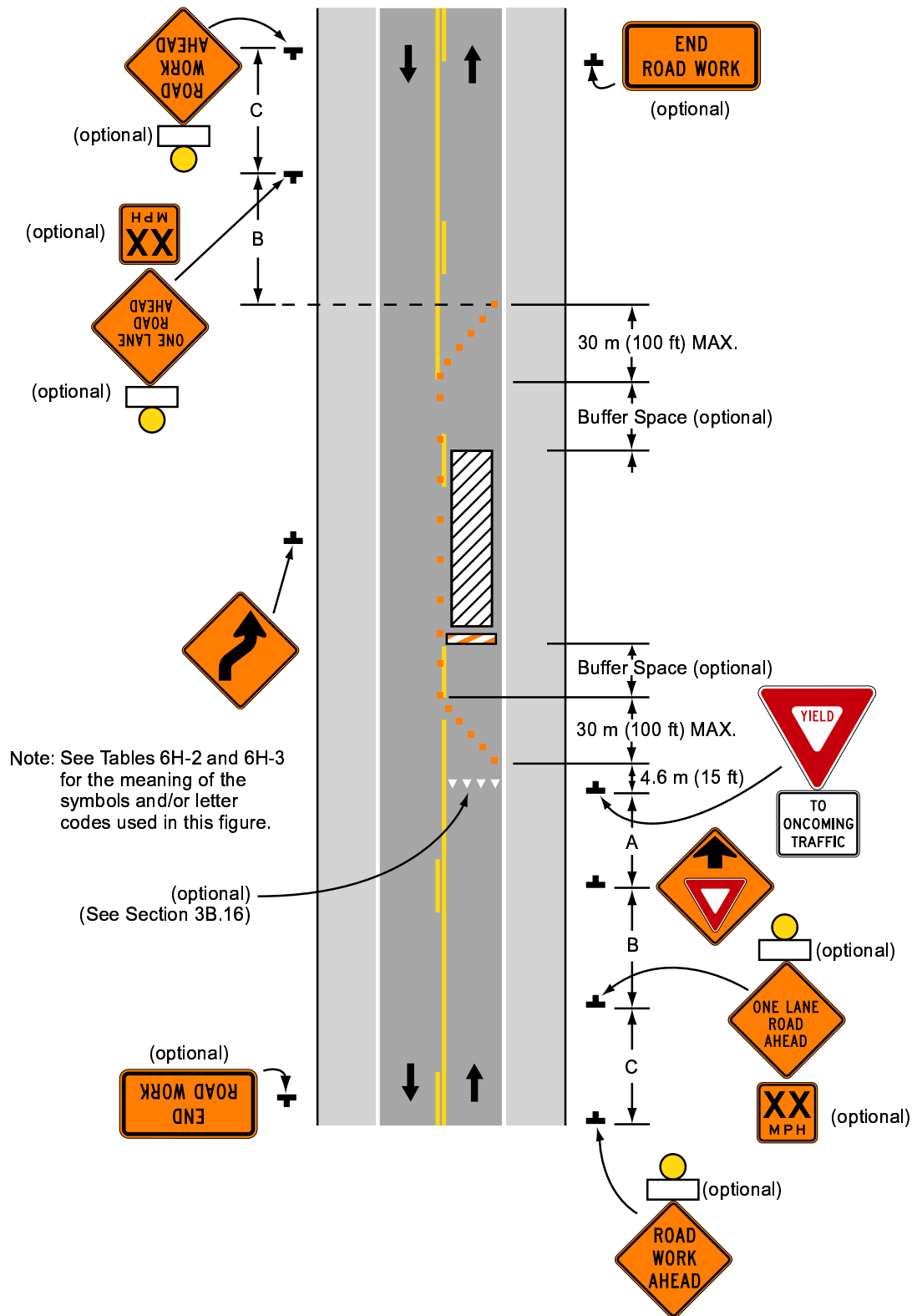
Figure 6H-11. Lane Closure on Two-Lane Road with Low Traffic Volumes (TA-11)
