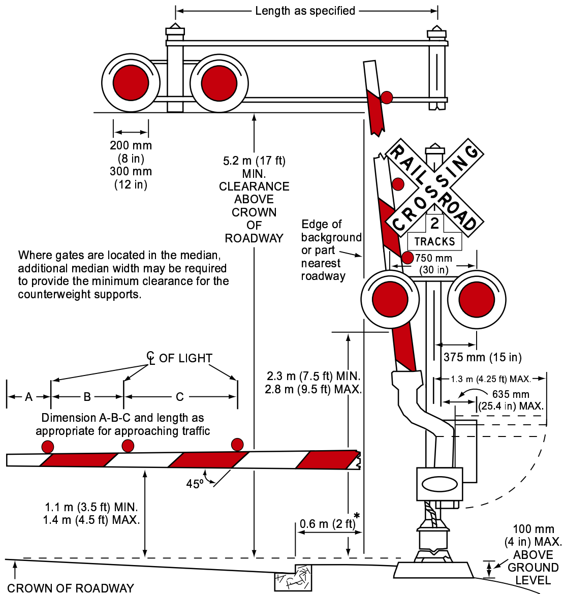
Figure 8D-1. Composite Drawing of Active Traffic Control Devices for Highway-Rail Grade Crossings Showing Clearance
