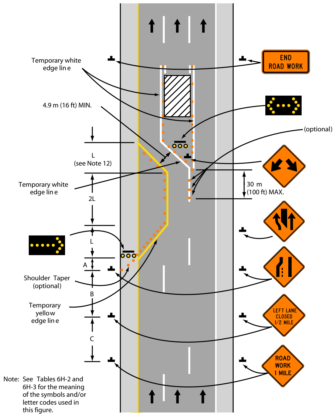
Typical Application 38
