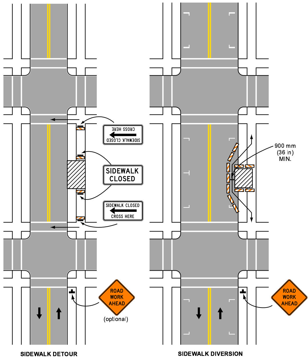
Typical Application 28
