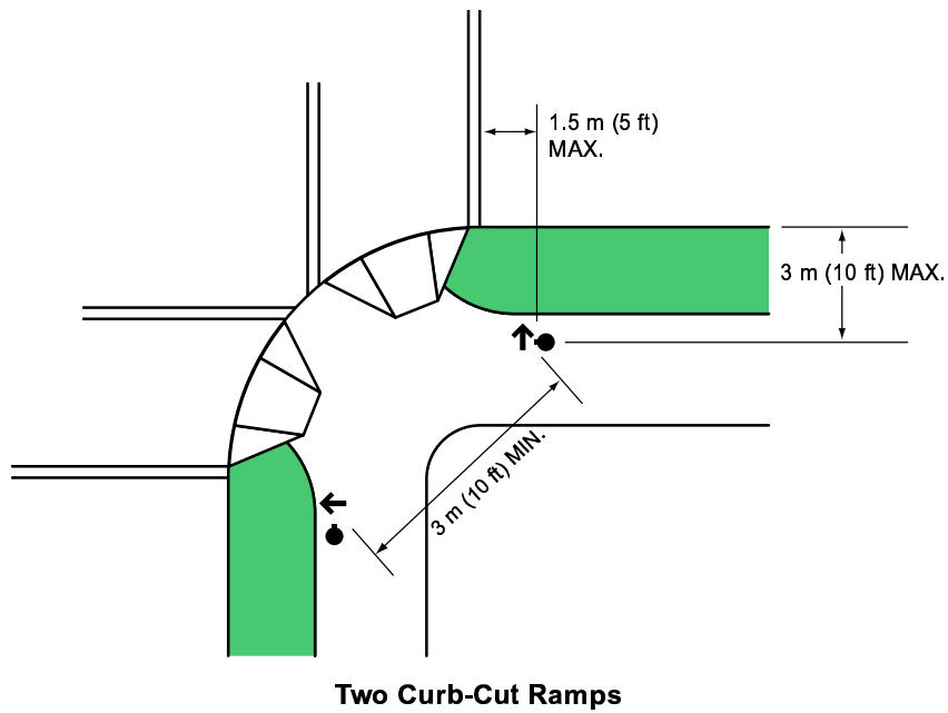
Figure 4E-2. Recommended Pushbutton Locations for Accessible Pedestrian Signals
