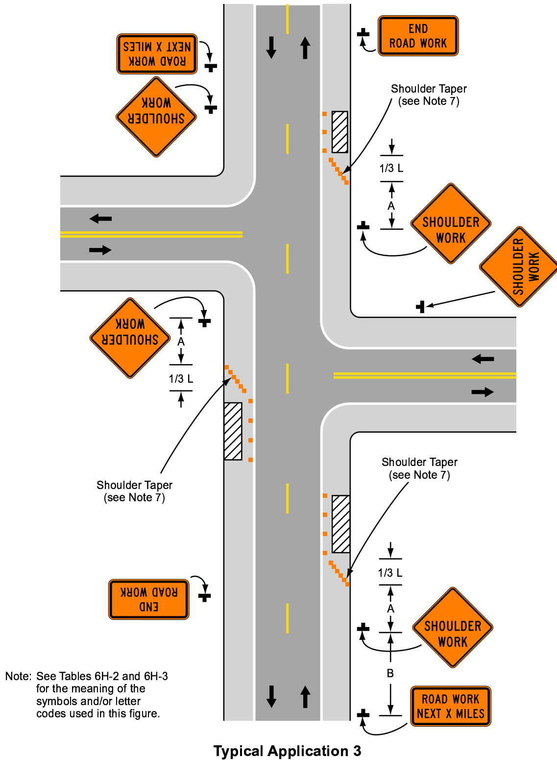
Figure 6H-3. Work on Shoulders (TA-3)
