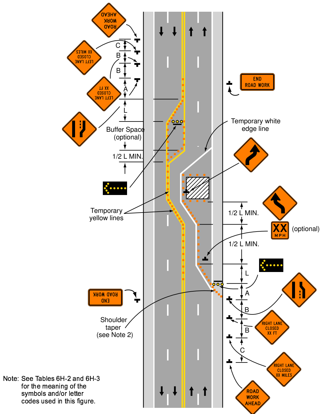
Typical Application 32
