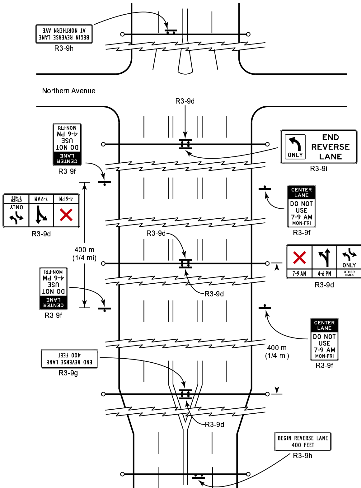
Figure 2B-6. Location of Reversible Two-Way Left-Turn Signs
