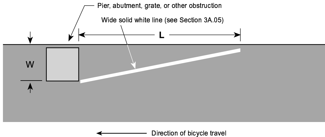
Figure 9C-8. Example of Obstruction Pavement Marking
