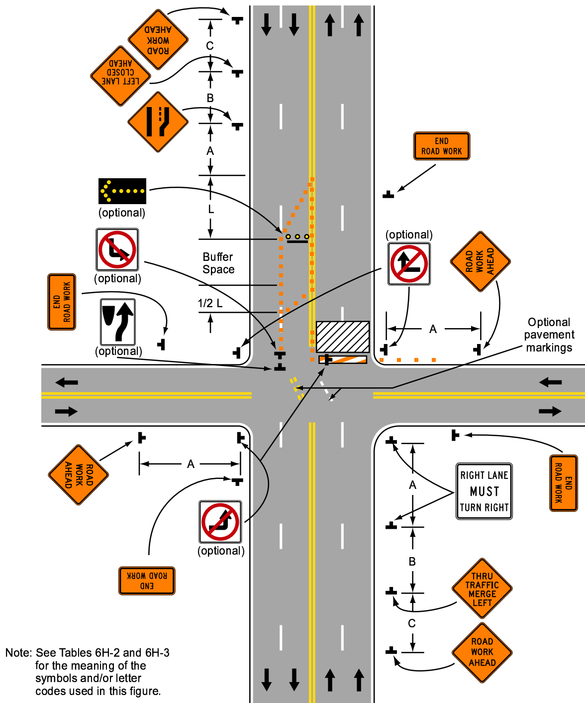
Typical Application 24
