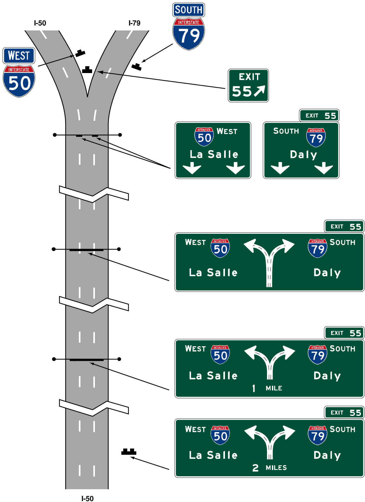
Figure 2E-5. Diagrammatic Signs for Split with Optional Lanes
