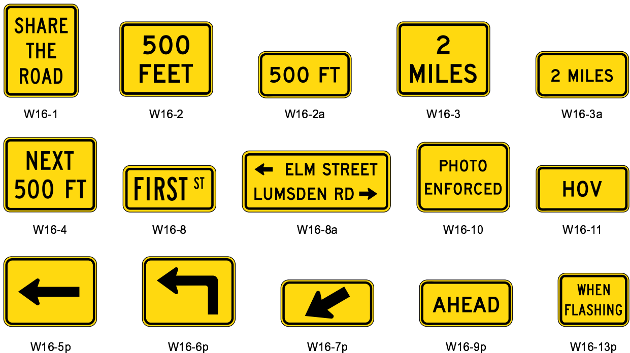
Figure 2C-11. Supplemental Warning Plaques
