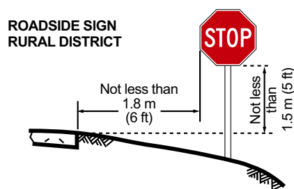
Figure 2A-1. Examples of Heights and Lateral Locations of Signs for Typical Installations
