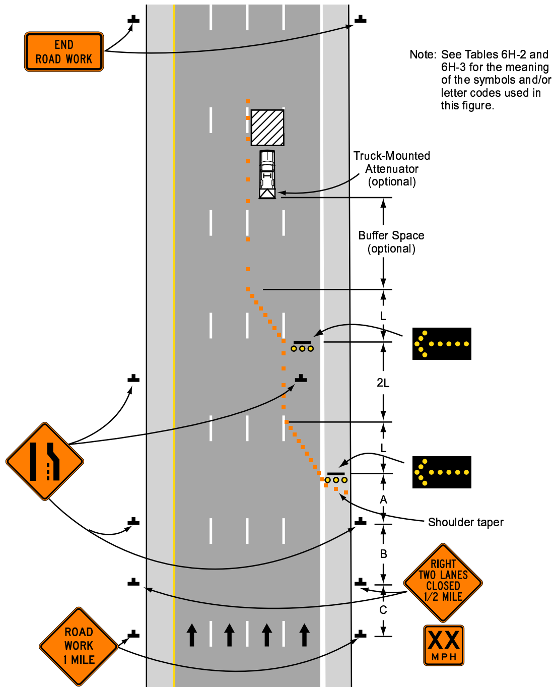
Typical Application 37
