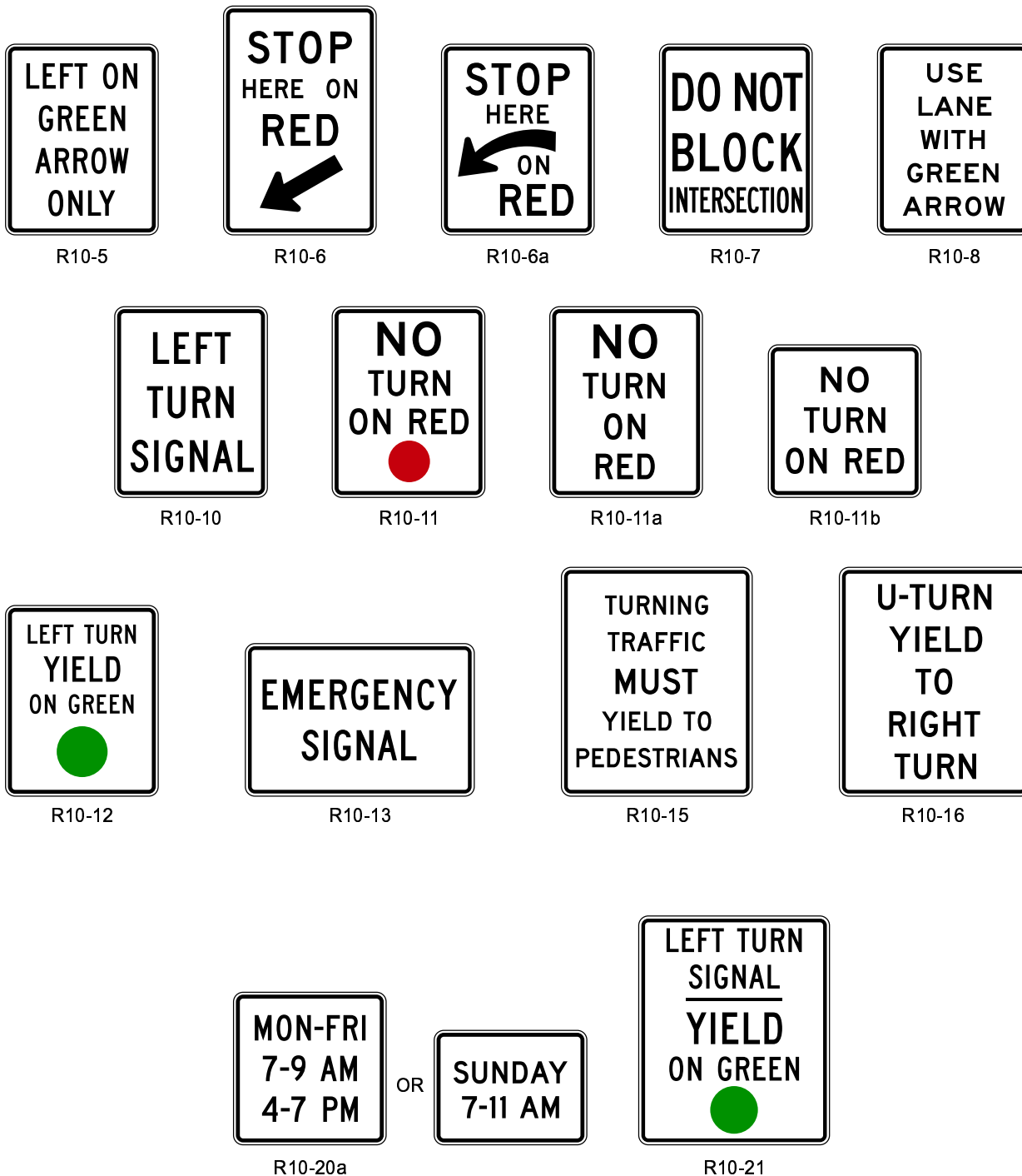
Figure 2B-19. Traffic Signal Signs
