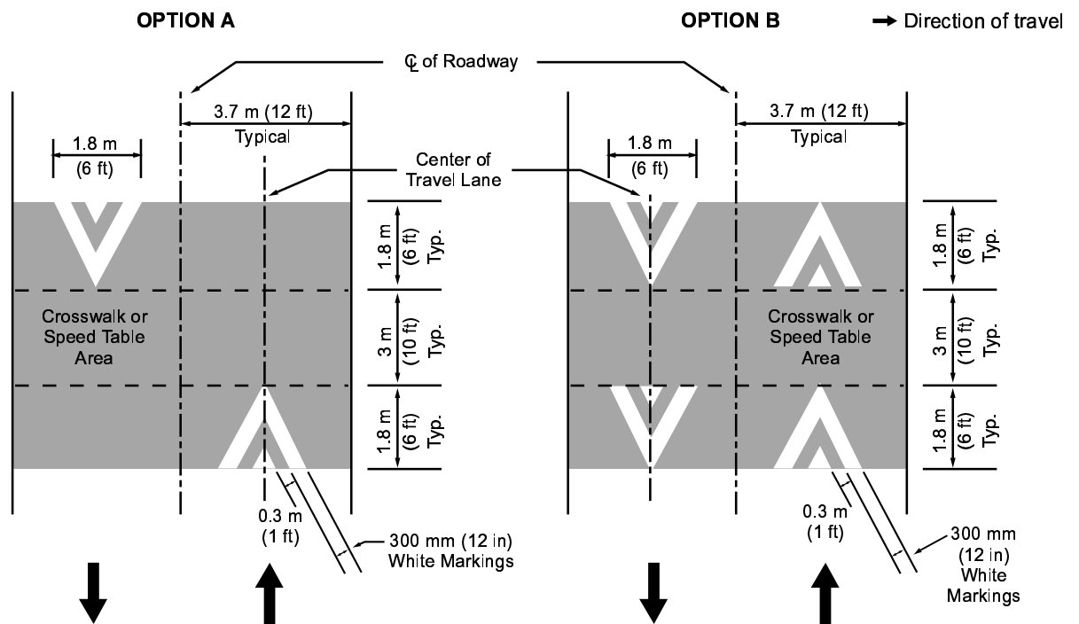
Figure 3B-30. Examples of Pavement Markings for Speed Tables or Speed Humps with Crosswalks
