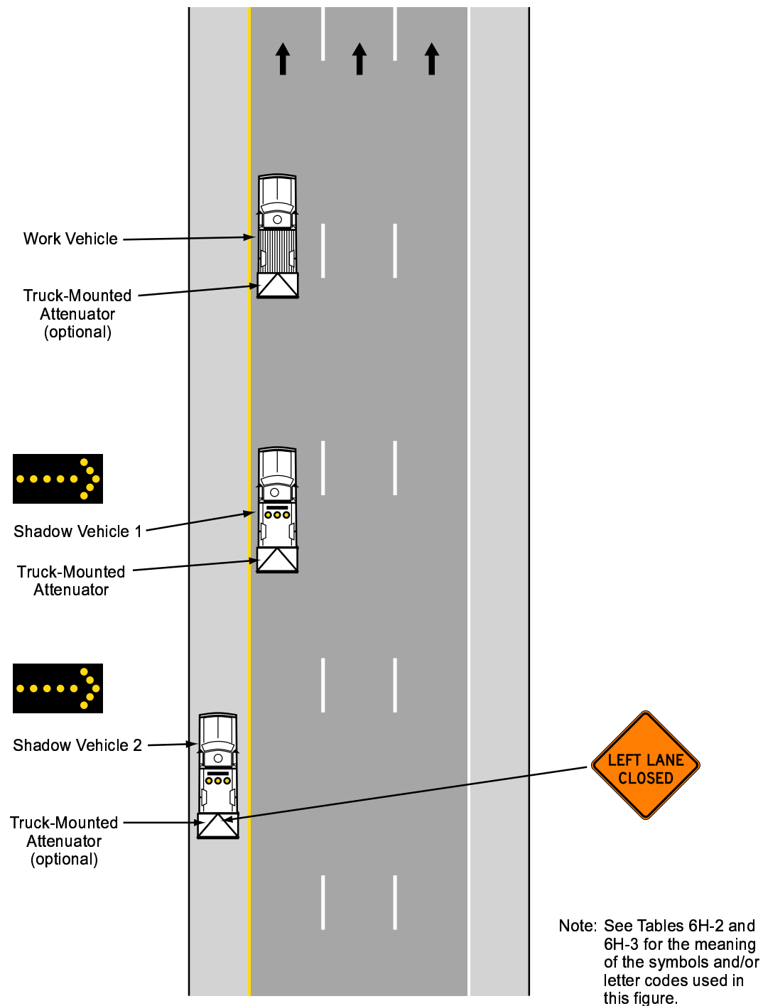
Typical Application 35
