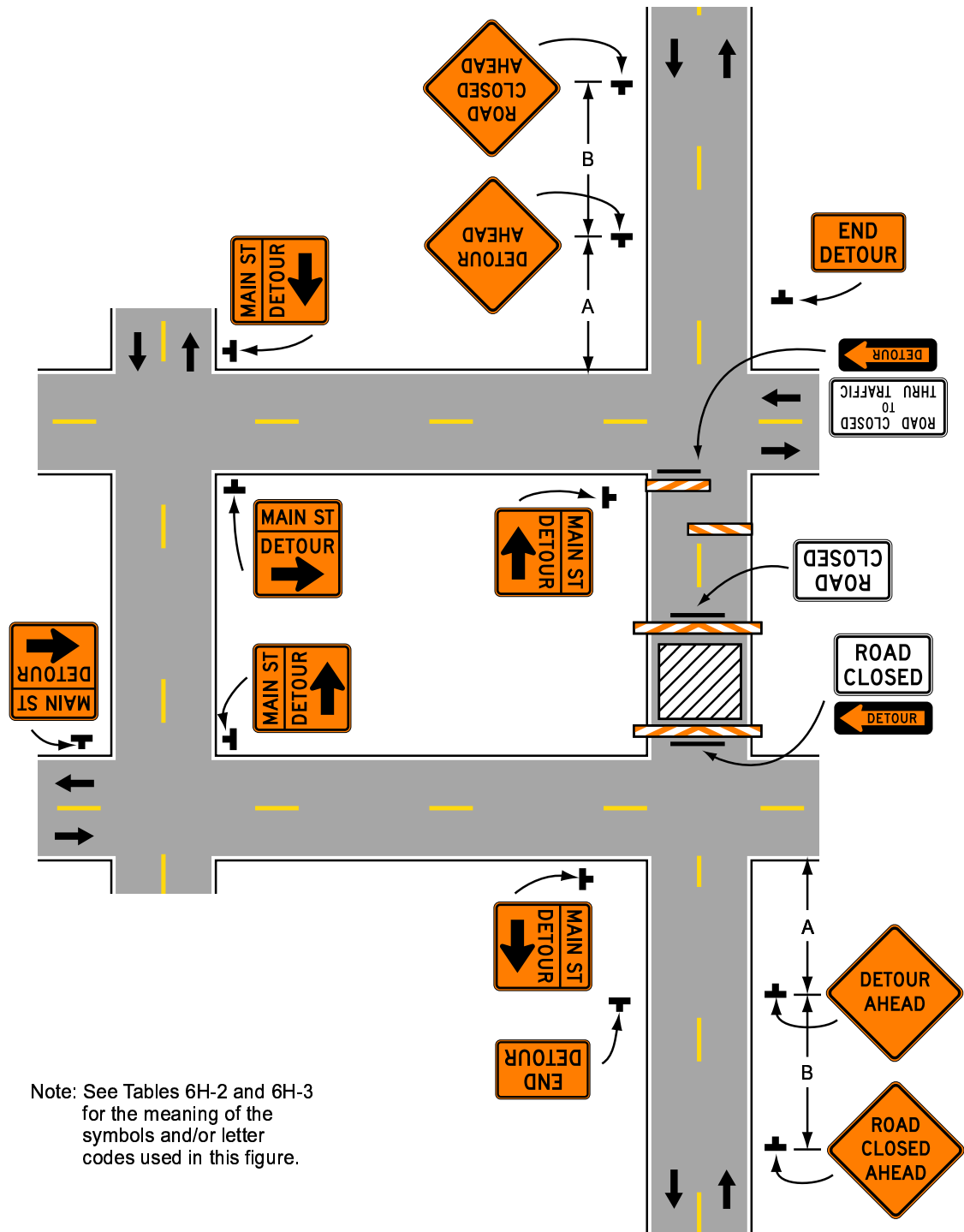
Typical Application 20
