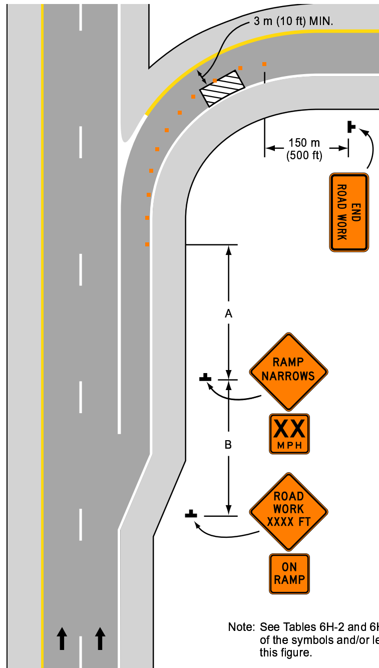
Typical Application 43
