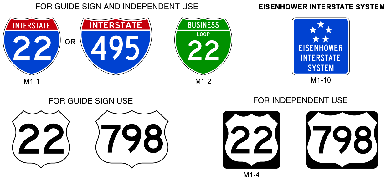
Figure 2E-11. Interstate and U.S. Route Signs
