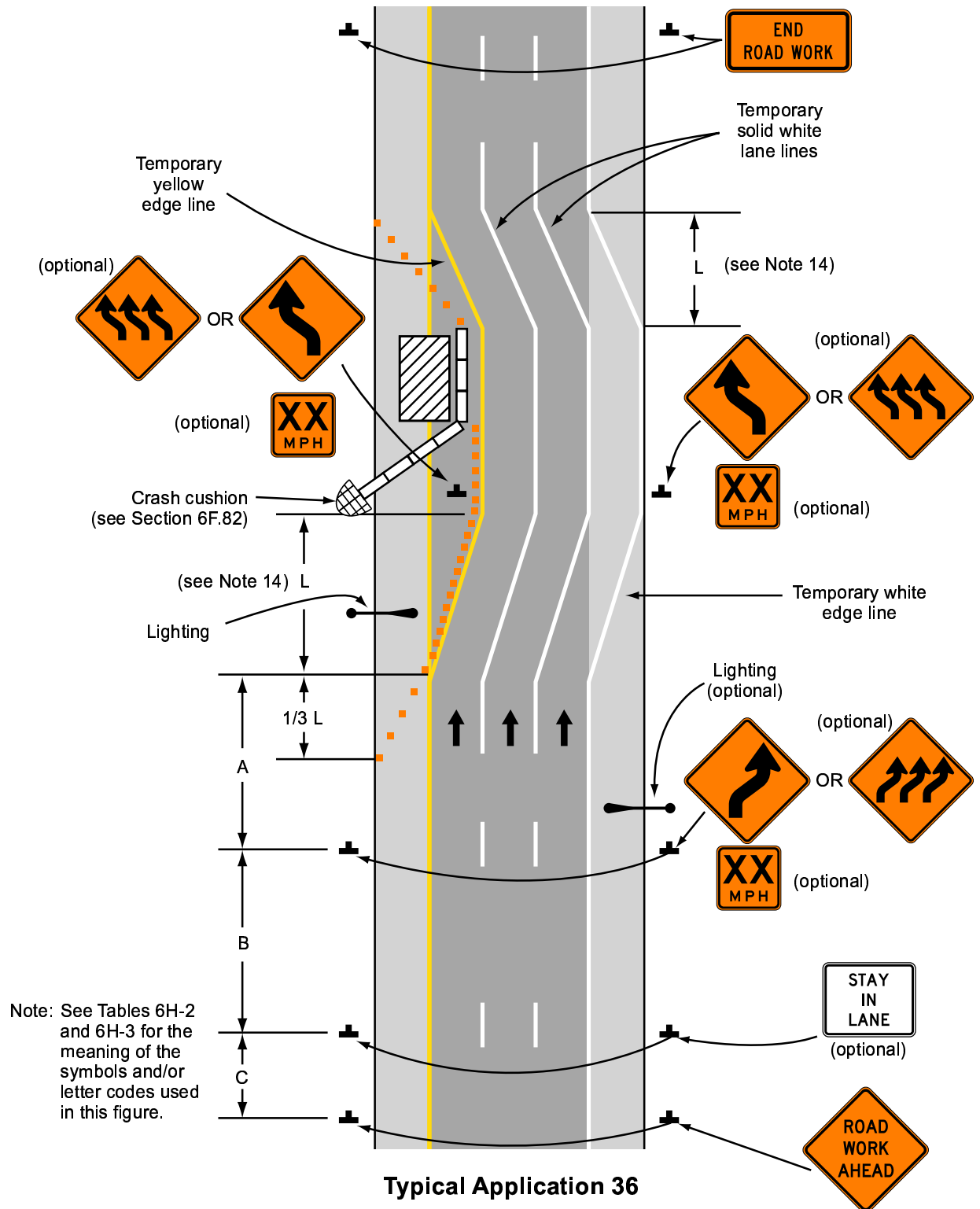
Figure 6H-36. Lane Shift on Freeway (TA-36)
