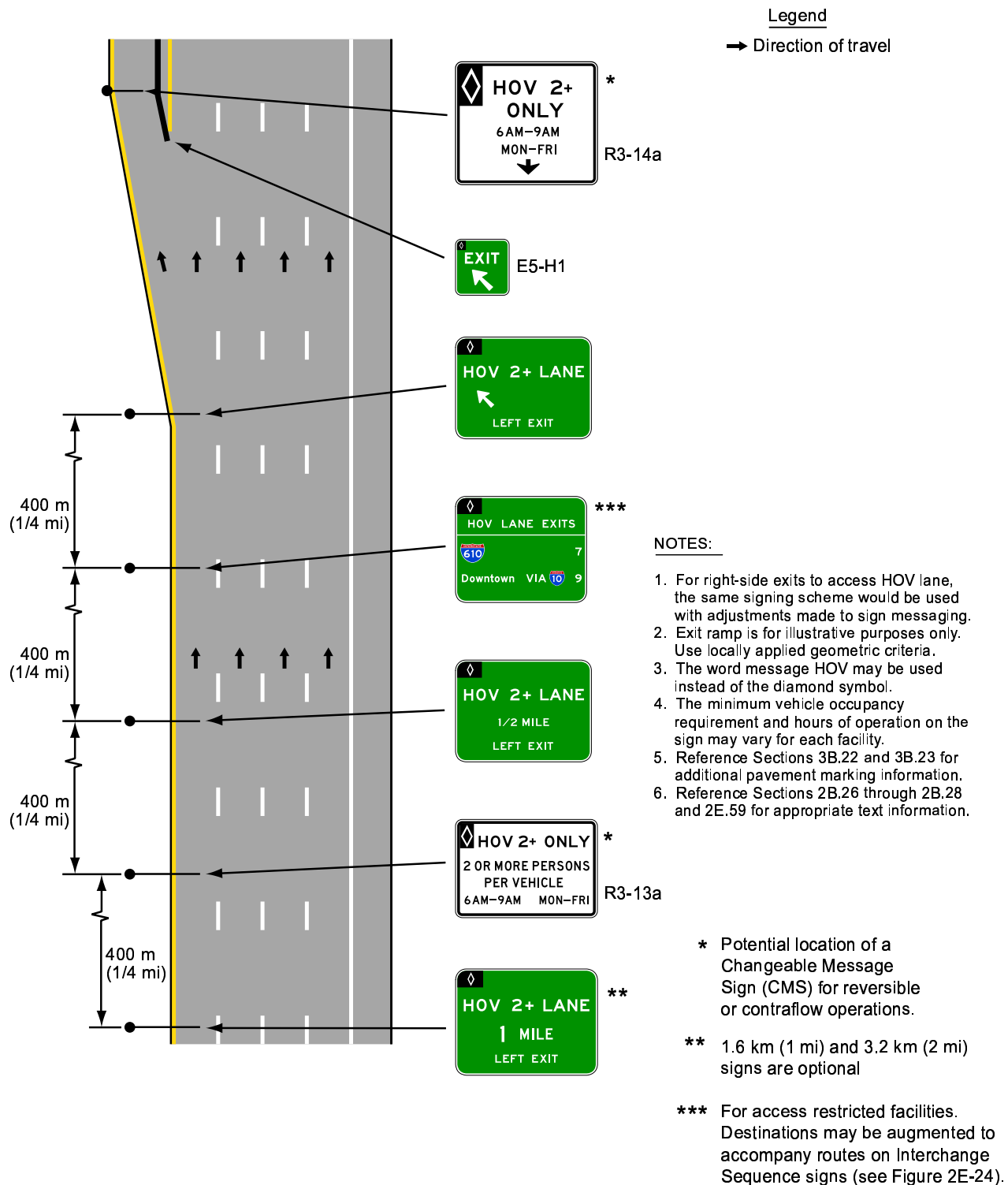
Figure 2E-46. Example of Signing for the Entrance to Barrier-Separated HOV Lanes
