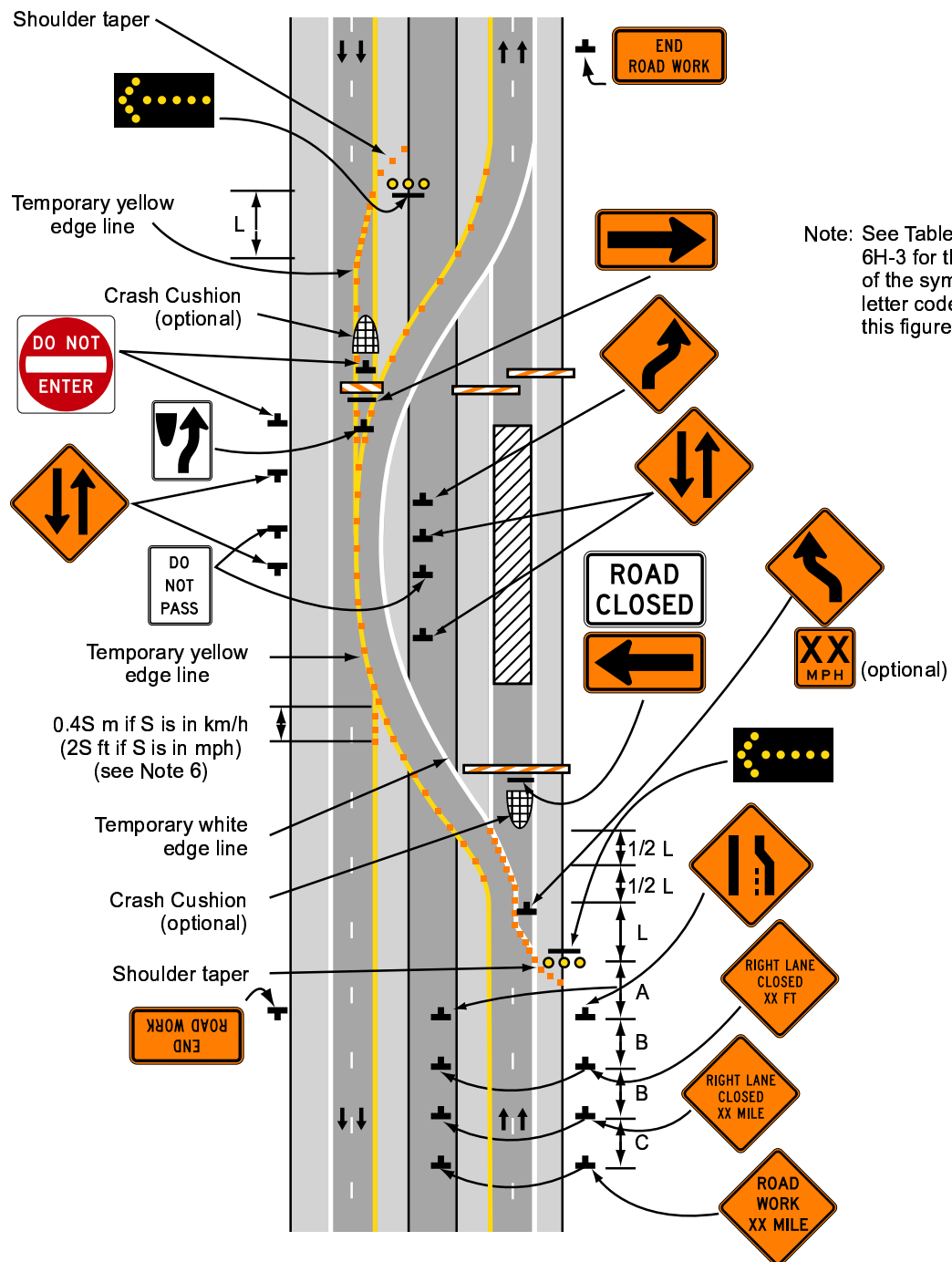
Typical Application 39
