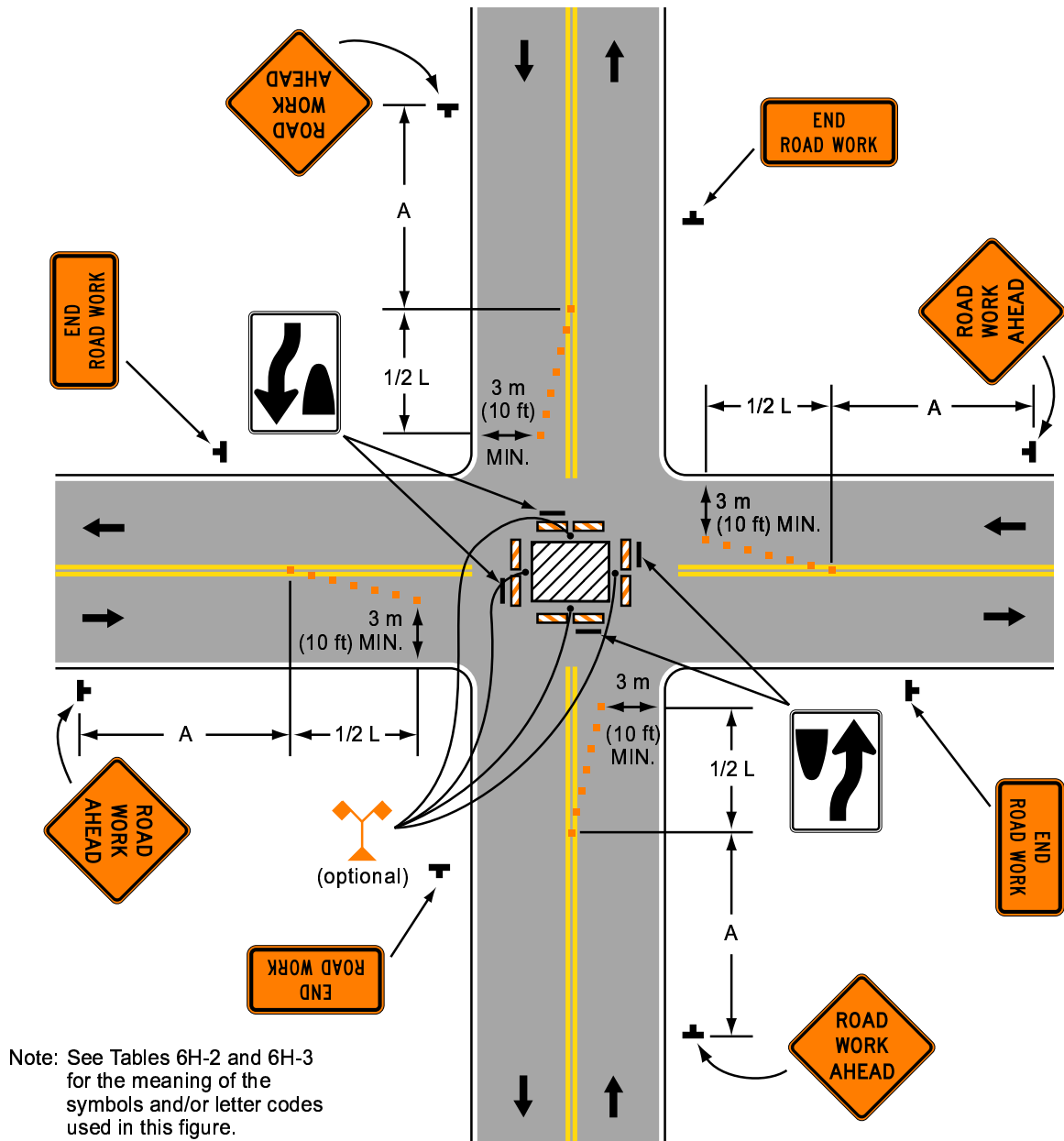
Typical Application 26
