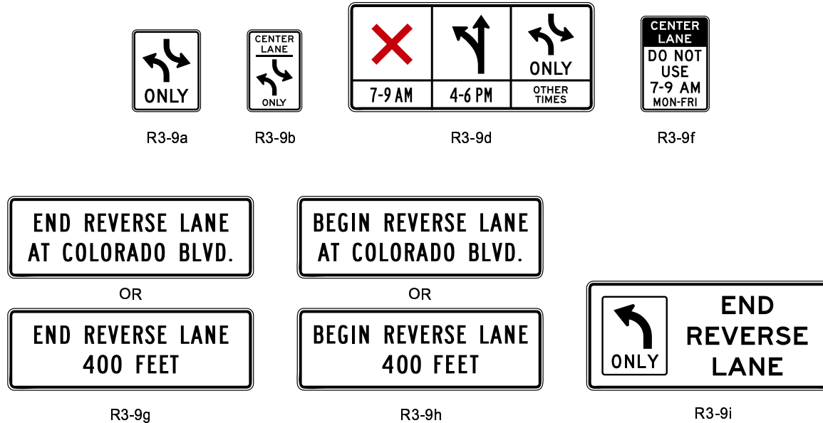
Figure 2B-5. Center and Reversible Lane Control Signs
