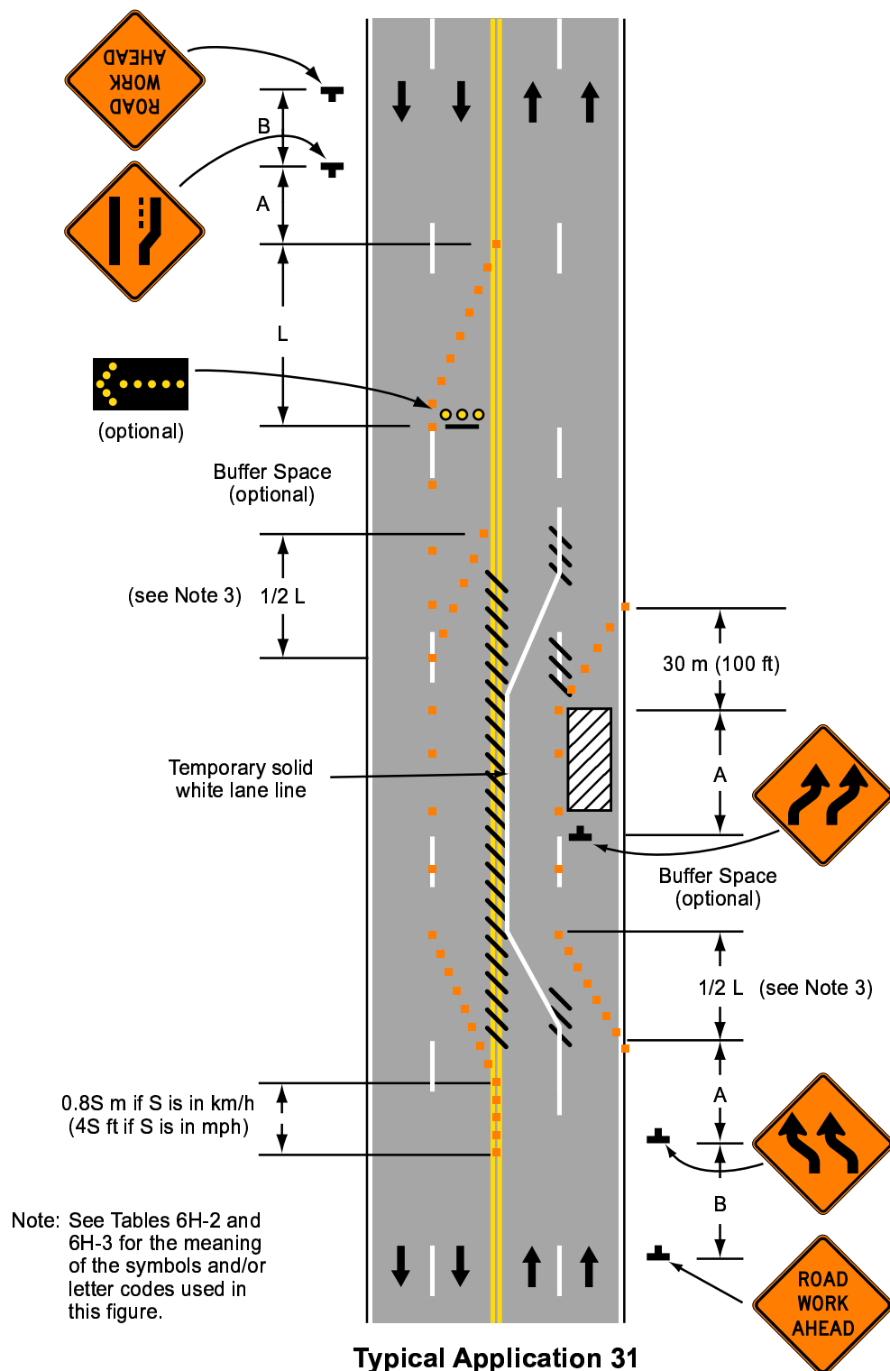
Figure 6H-31. Lane Closures on Street with Uneven Directional Volumes (TA-31)
