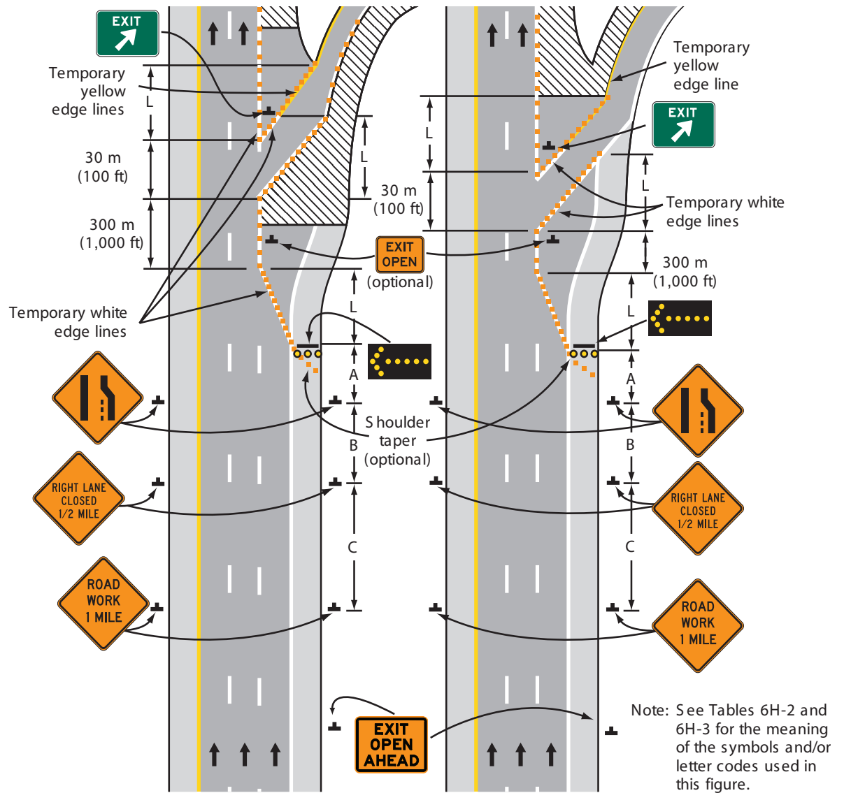
Typical Application 42
