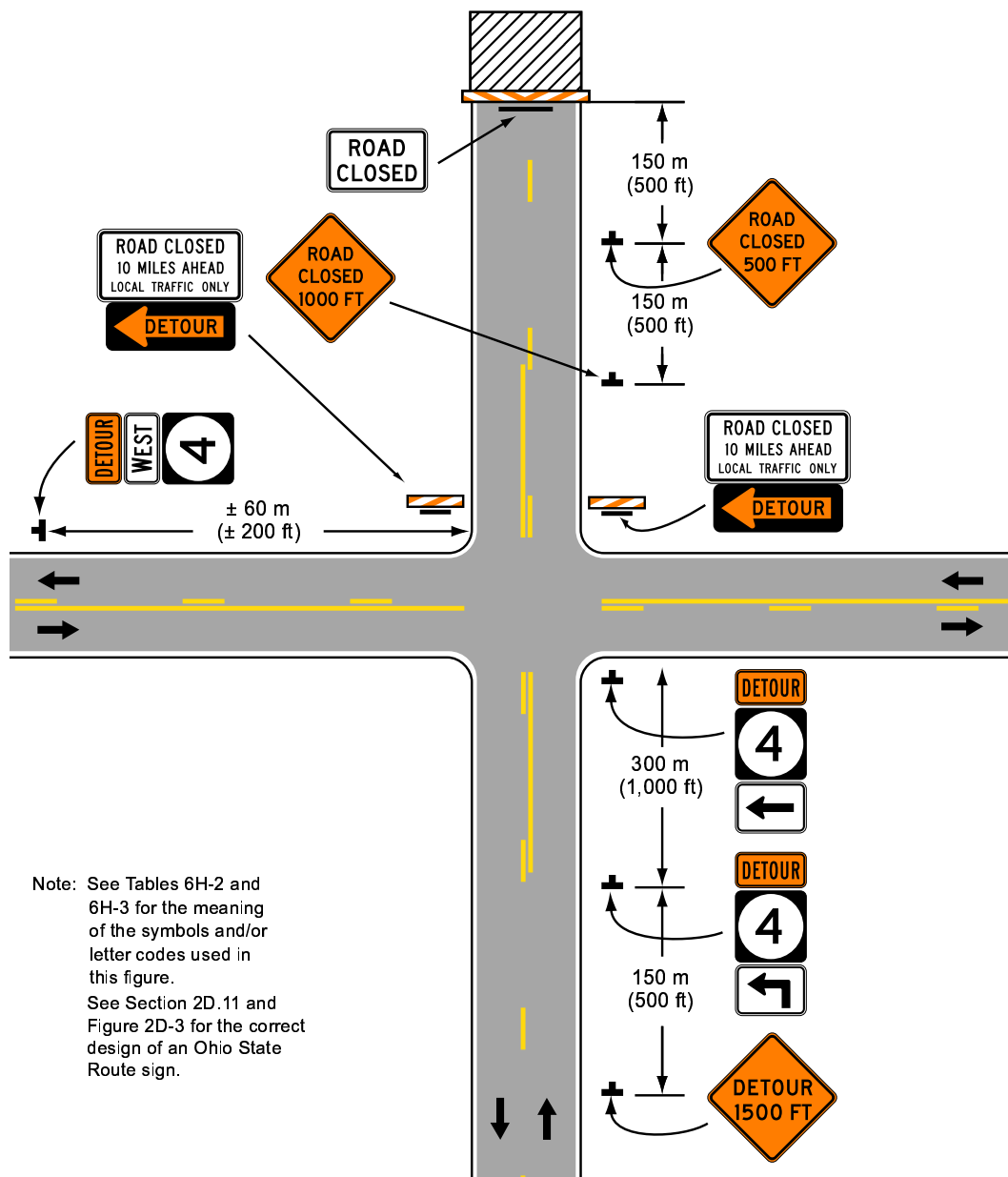
Typical Application 8
