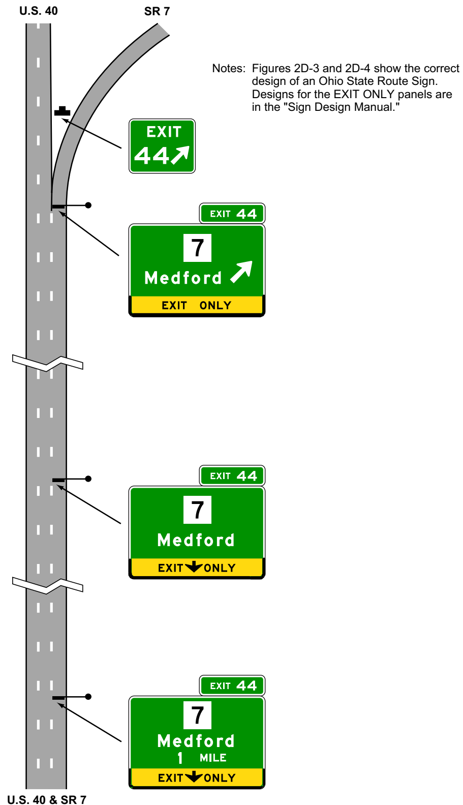
Figure 2E-10. EXIT ONLY Panels for Right Lane Dropped at an Interchange
