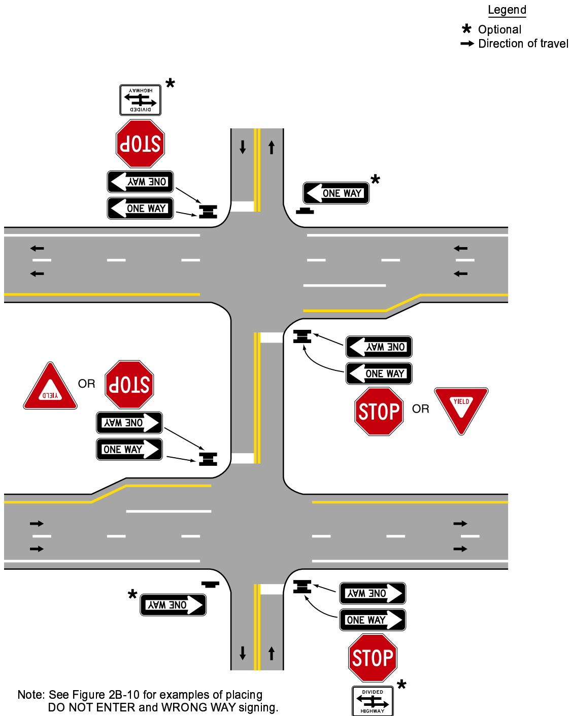
Figure 2B-13. Examples of ONE WAY Signing for Divided Highways with Medians of 9 m (30 ft) or Greater
