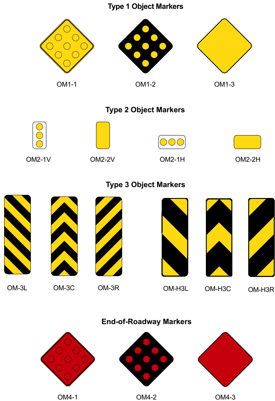
Figure 3C-1. Object Markers and End-of-Roadway Markers
