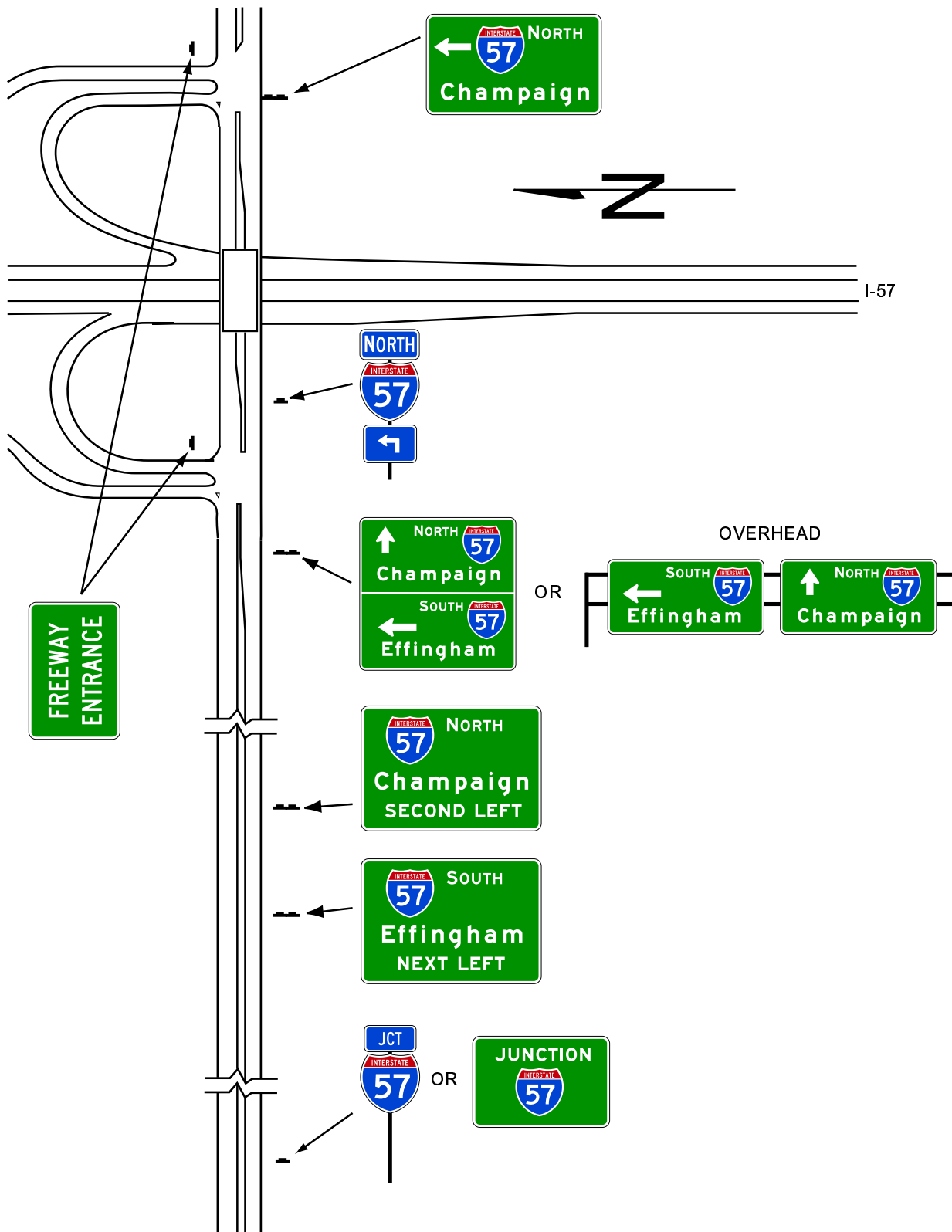
Figure 2E-37. Examples of Multi-lane Crossroad Signing for Partial Cloverleaf Interchange
