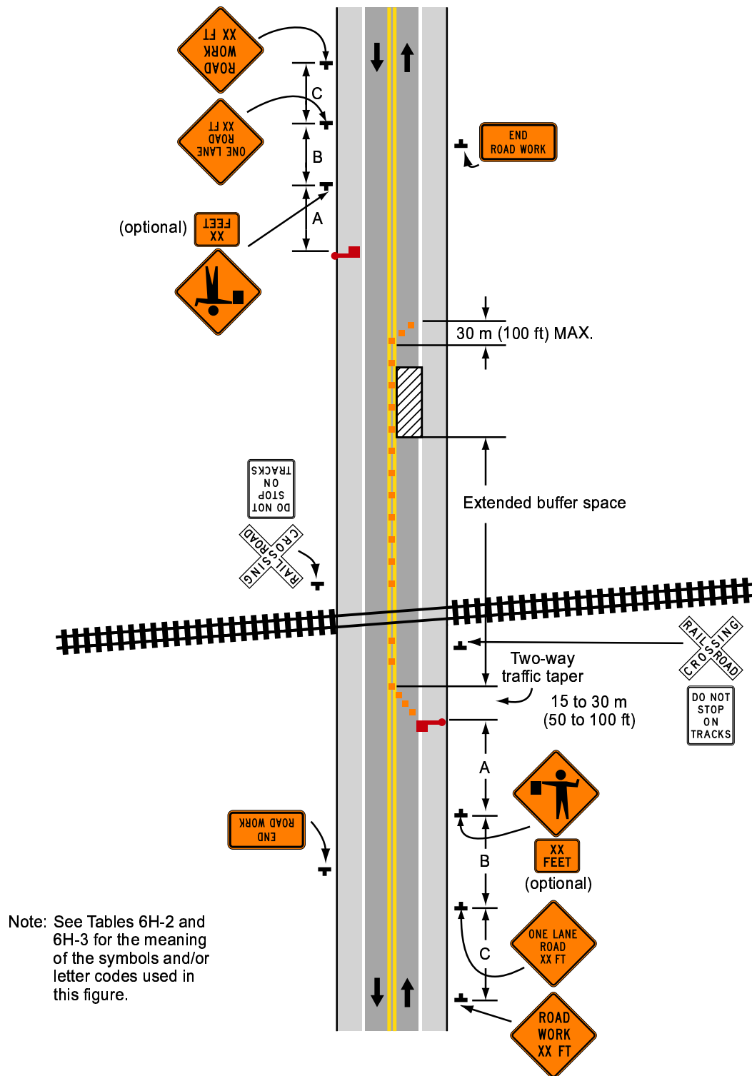
Typical Application 46
