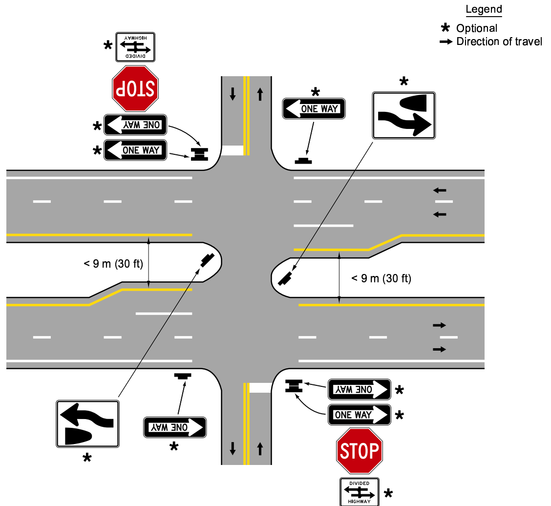
Figure 2B-14. Examples of ONE WAY Signing for Divided Highways with Medians Less Than 9 m (30 ft)
