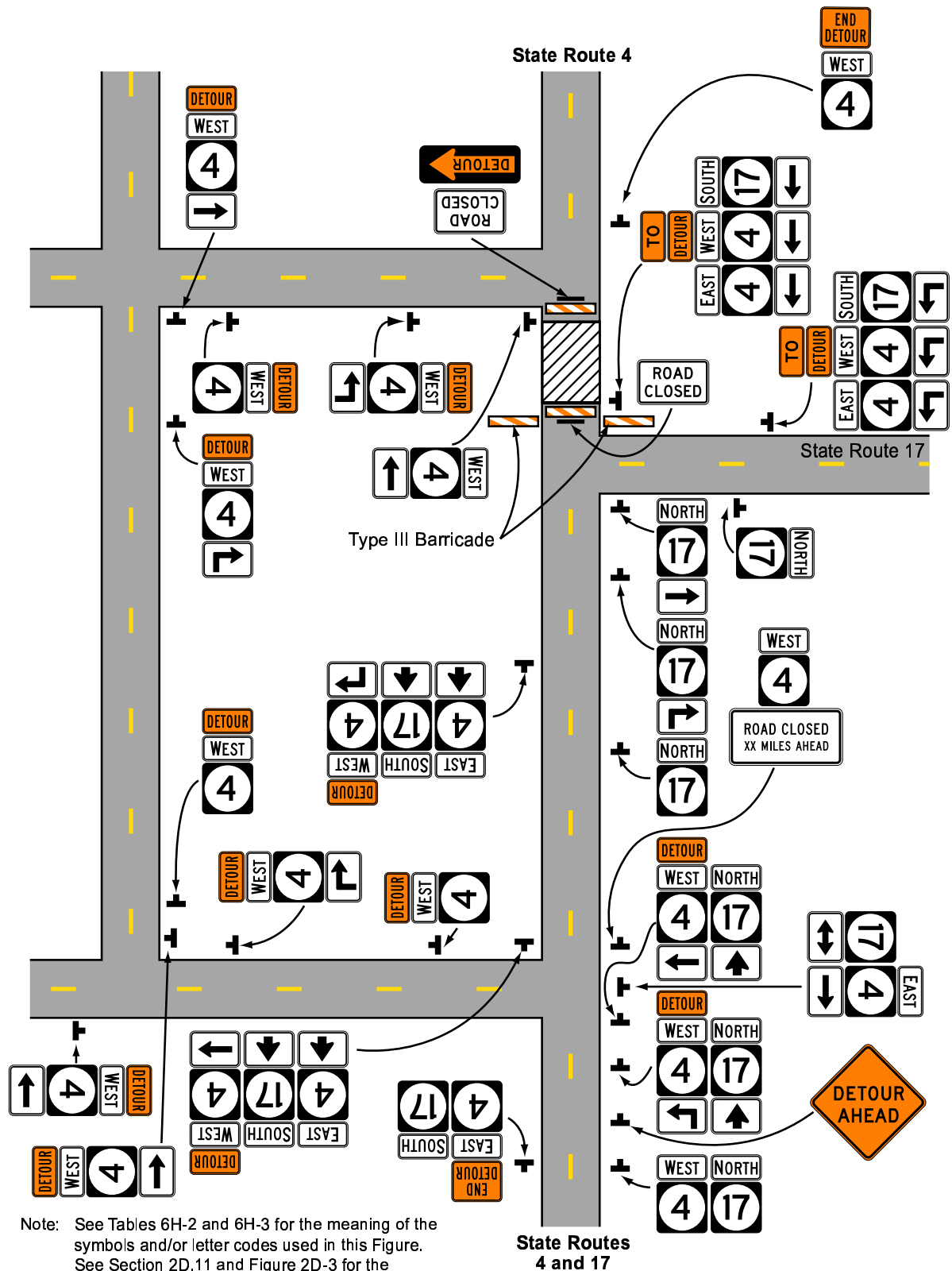
Figure 6H-9. Overlapping Routes with Detour (TA-9)
