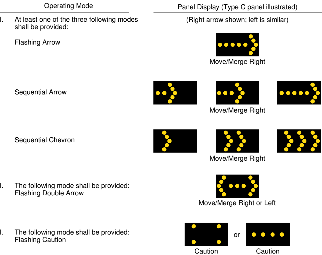
Figure 6F-6. Advance Warning Arrow Display Specifications
