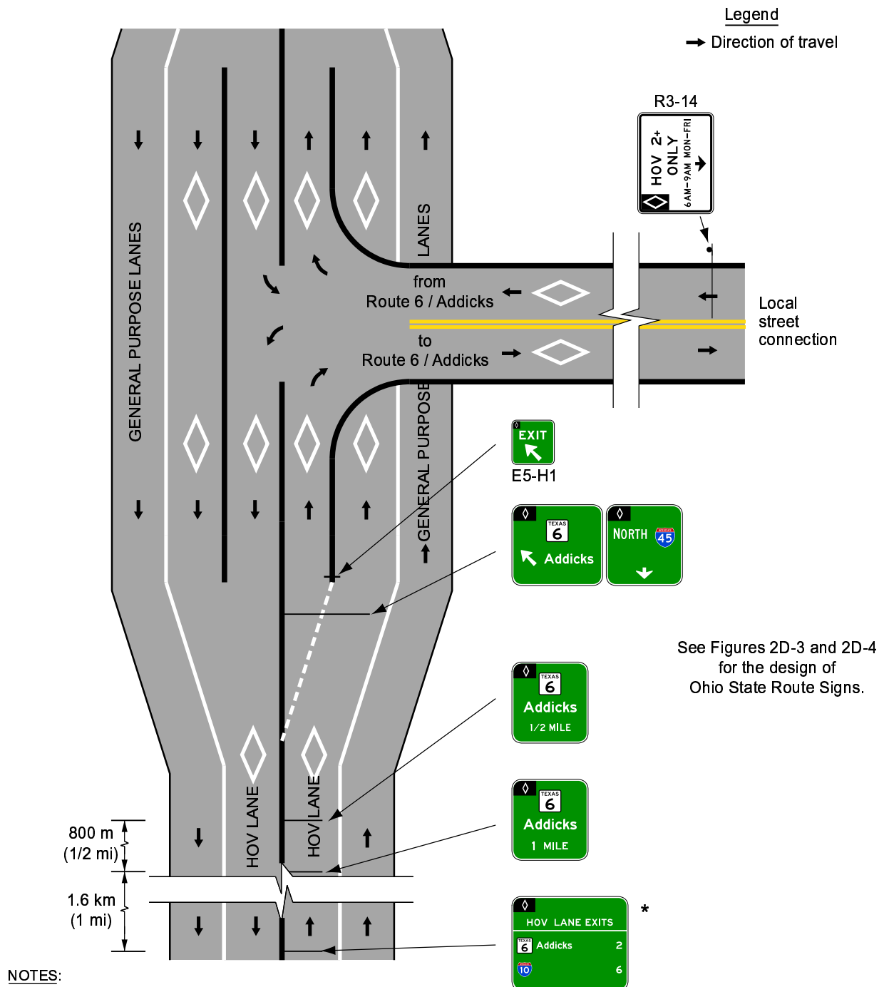
Figure 2E-51. Example of Signing for a Direct Access Ramp to an HOV Lane from a Local Street
