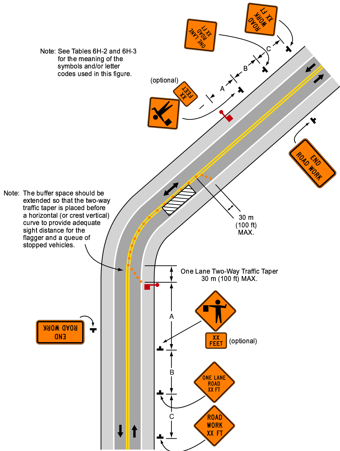
Typical Application 10
