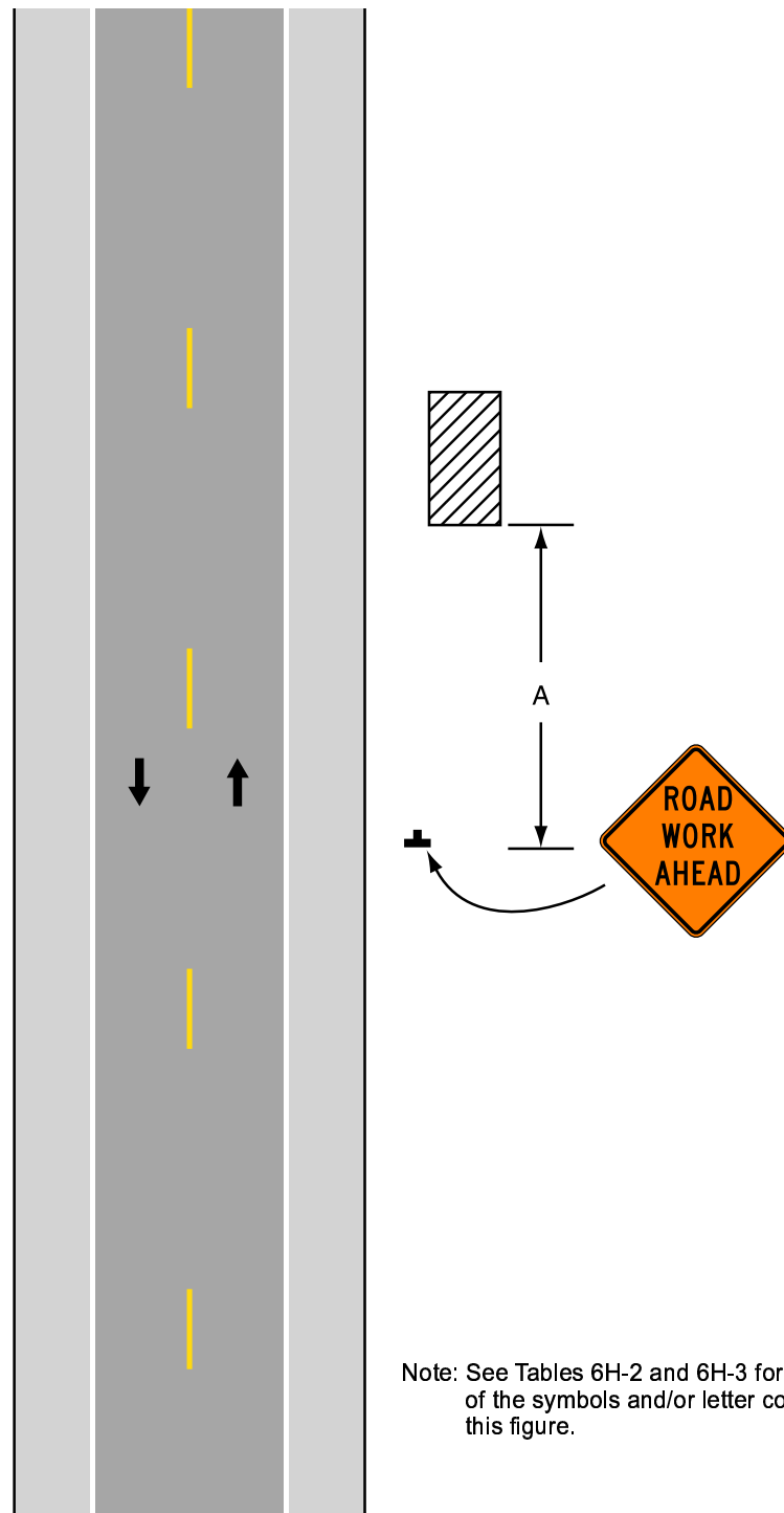
Typical Application 1
