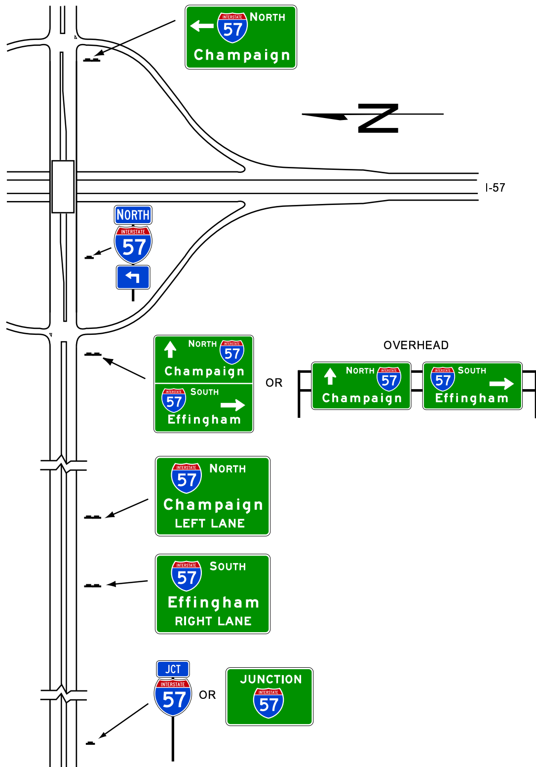
Figure 2E-36. Examples of Multi-lane Crossroad Signing for Diamond Interchange
