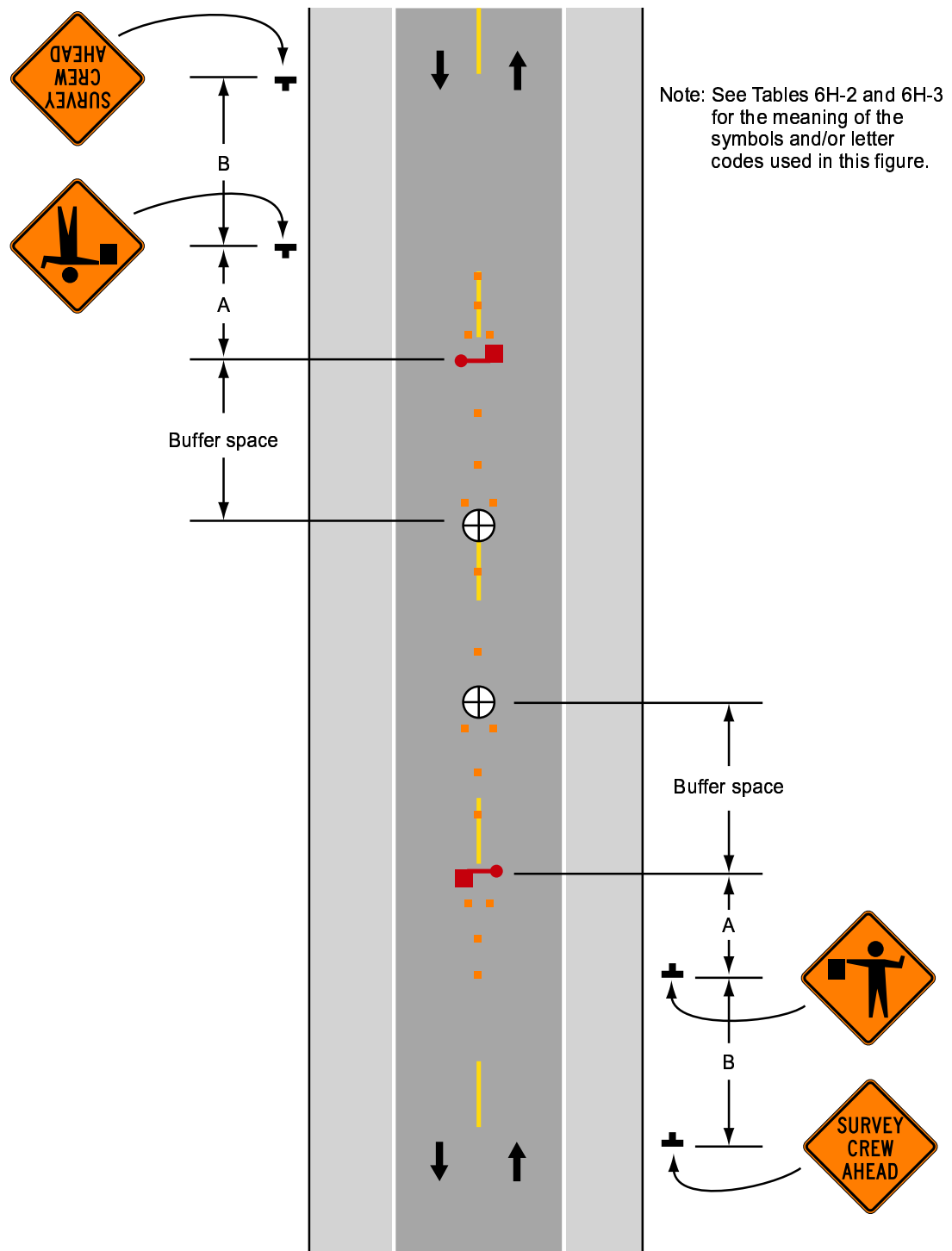
Typical Application 16
