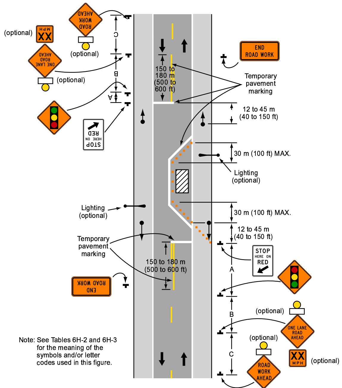
Typical Application 12
