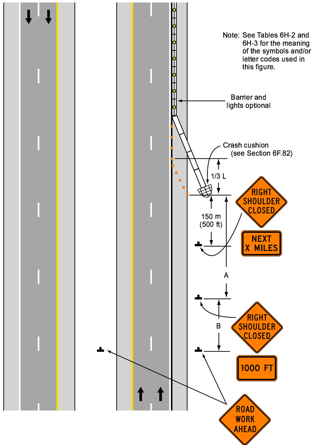
Typical Application 5
