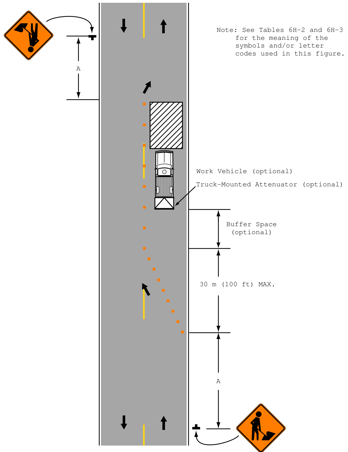
Typical Application 18
