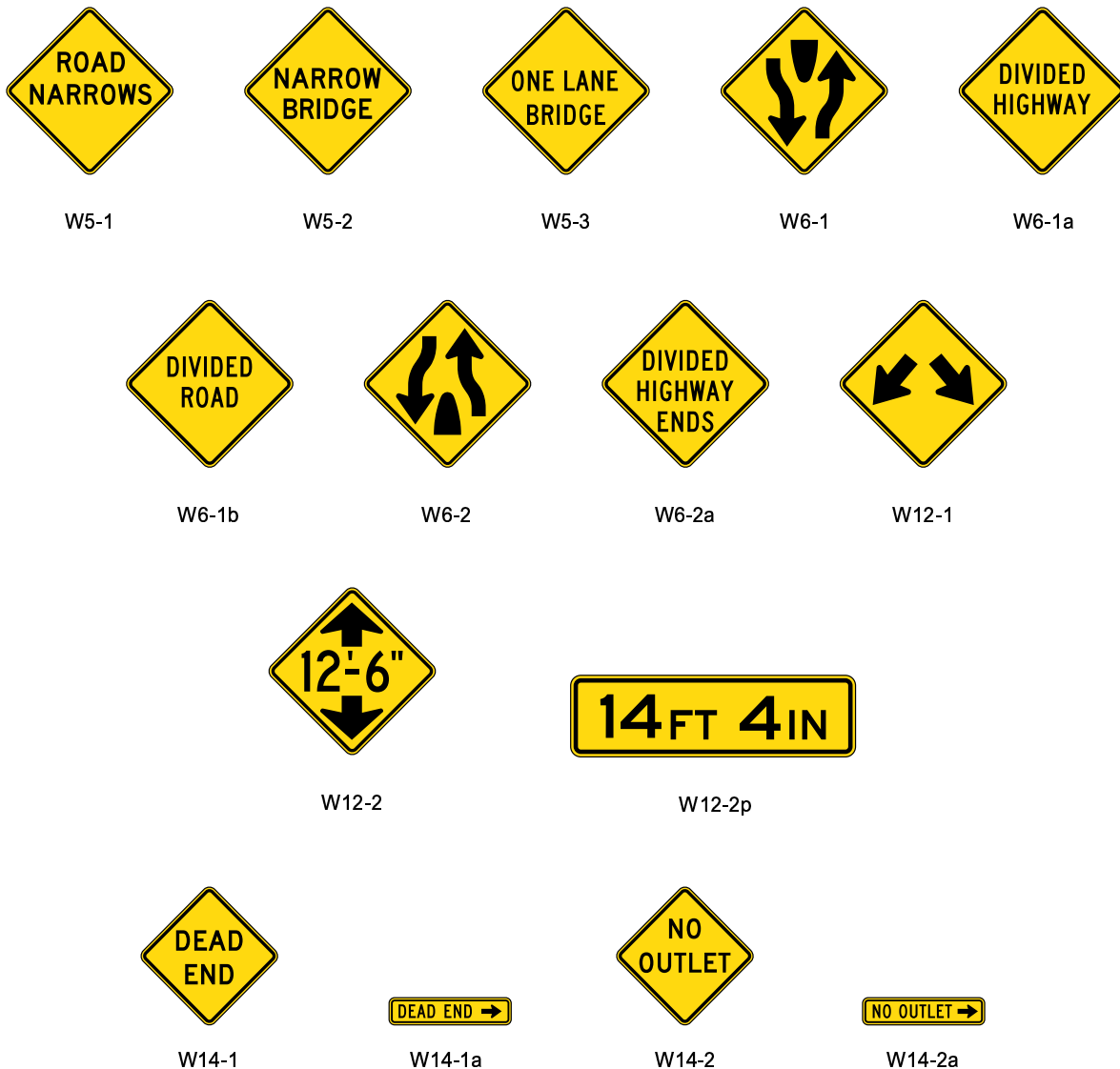
Figure 2C-3. Miscellaneous Warning Signs
